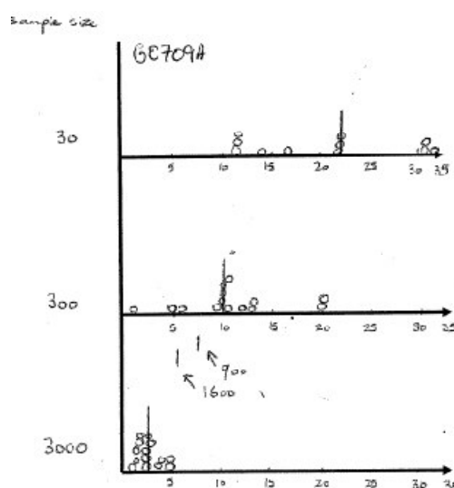
Figure 4.7. Student G0709A given as part of a relational response.
