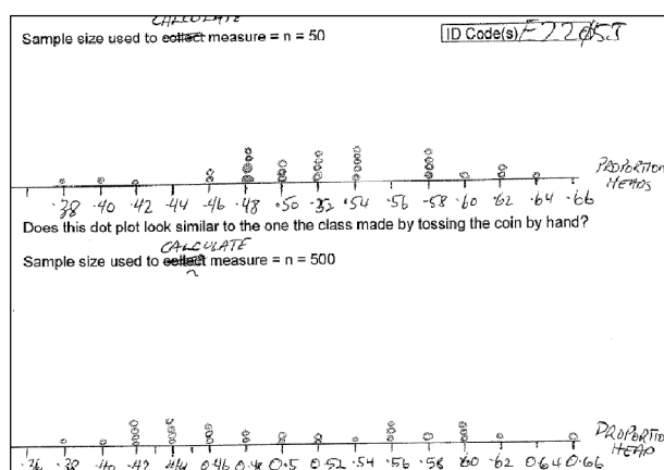
Figure 4.11. Student E2205J, proportion of heads for samples size of 50 & 500 tosses of a coin, prestructural response.
