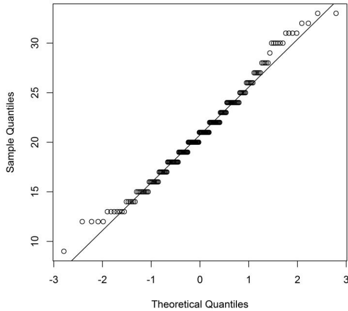
Figure 15. Normal Q-Q plot for post-test scores in low conformity classrooms
