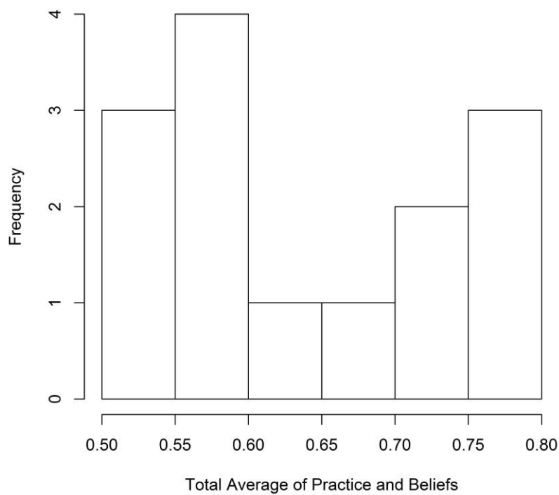
Figure 11. Histogram of total average conformity to SRLE conformity.
