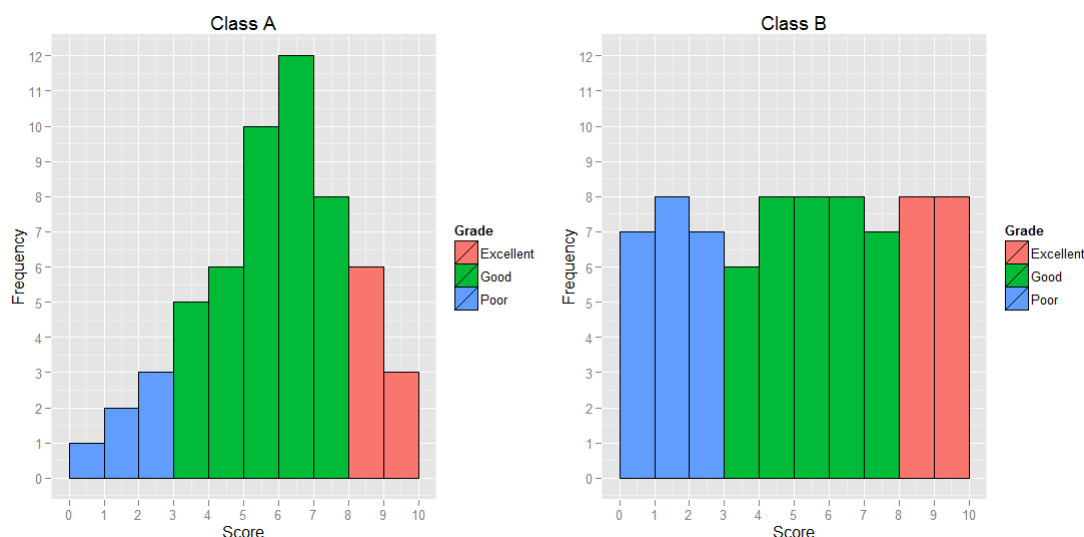
Figure 3.2: Item 9- Test Scores for Large-Test Histogram
