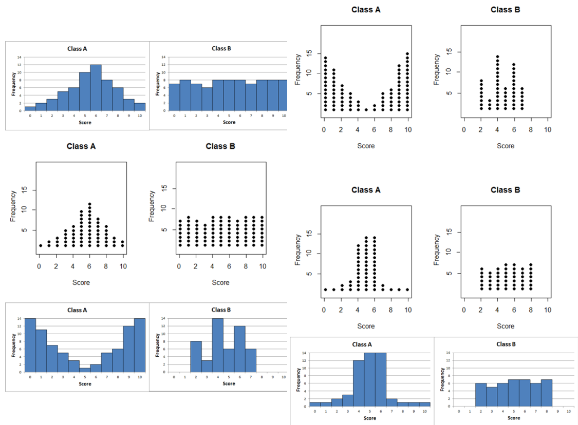
Figure 7.6: Item 6- Test Score Variability Combination
